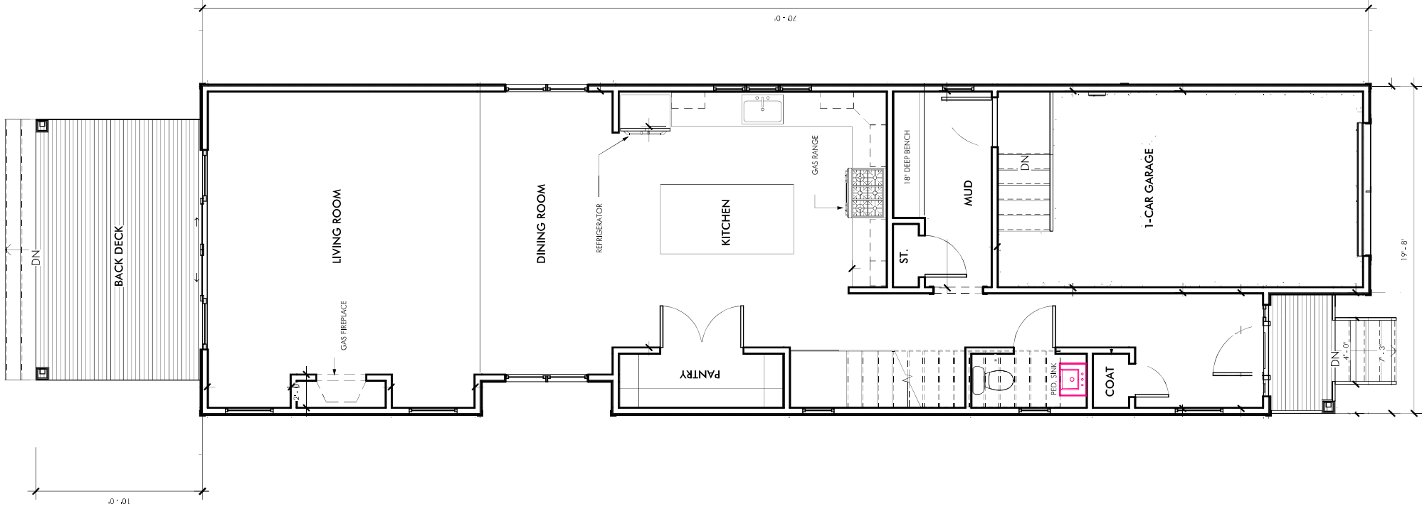
First Floor
