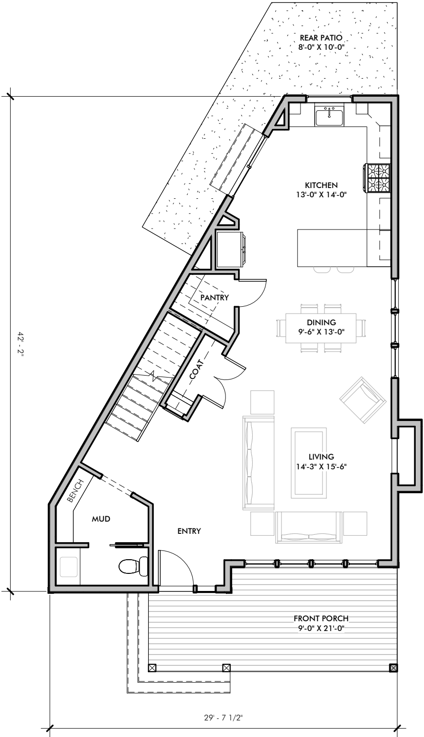
FIRST FLOOR PLAN 1/8" = 1'-0"
