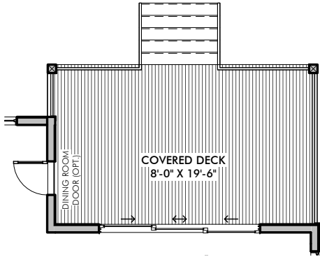
LIVING ROOM SLIDER OPTION 1" = 10'-0"
