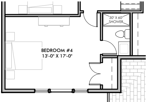
4TH BEDROOM WITH BATH OPTION 1" = 10'-0"
